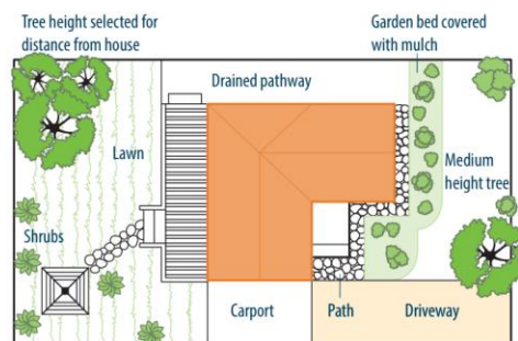
FIGURE 2 Gardens for a reactive site.
